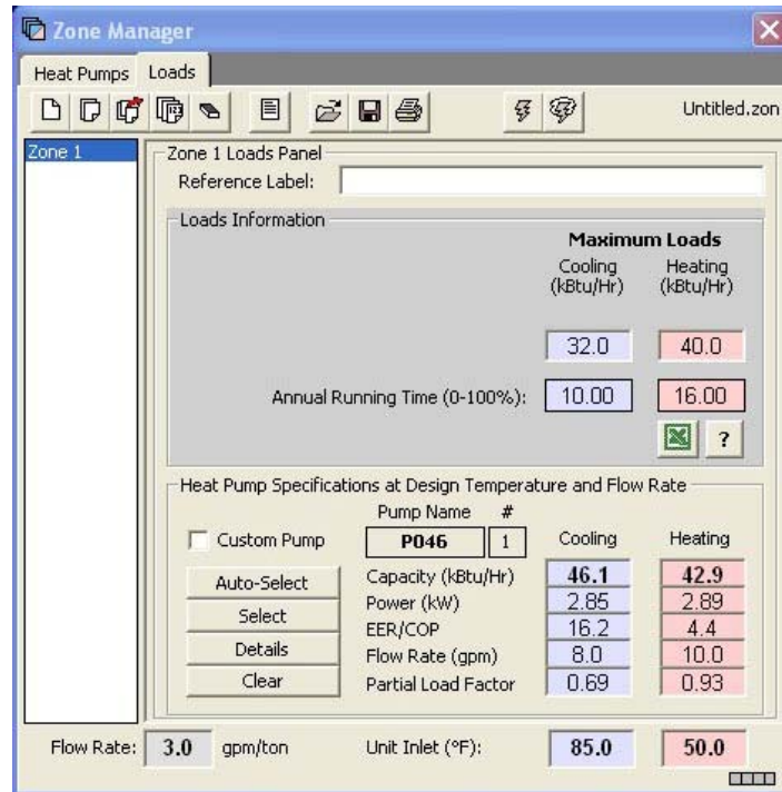
Zone Manager Loads Module: Ready for Heat Exchanger Design
