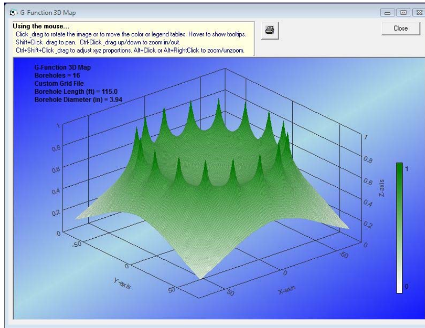
Fig. 4.7 A G Map for a Circular Loopfield
