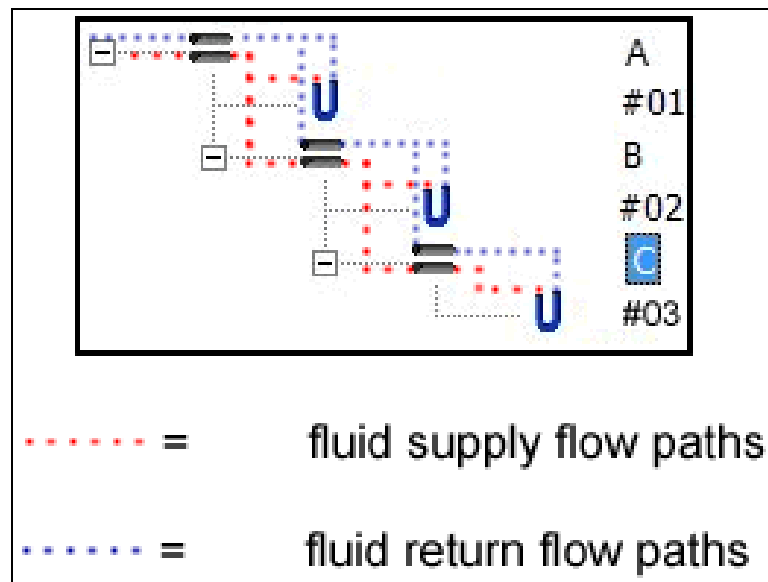
Fig. 11.53 Fluid Flow Paths of the Direct Return GHX Module
