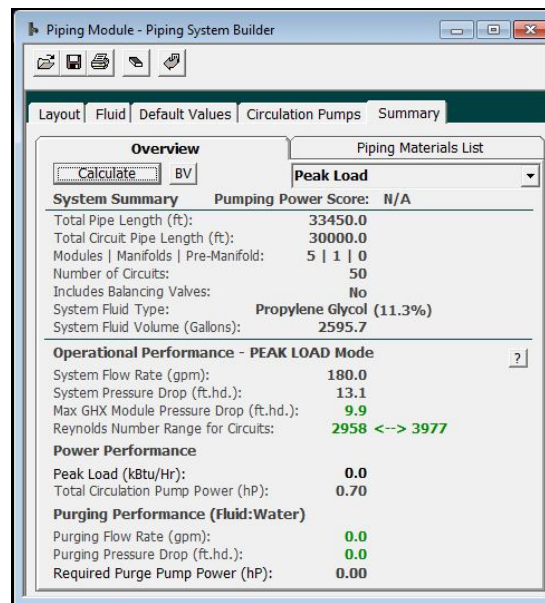
Fig. 11.121 No Balancing Valves Yet
